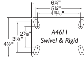
* Attaching Bolt Size For Plate 1/2" (Formerly 125L)
