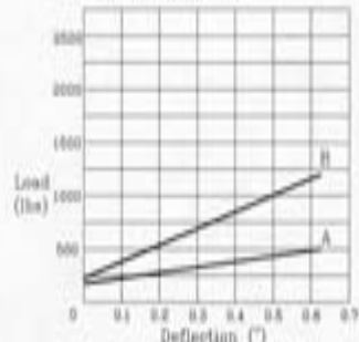
Deflection Chart SSL7063(RSL7063)
