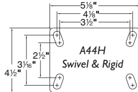
* Attaching Bolt Size For Plate 3/8" (Formerly 125F)
