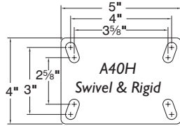
* Attaching Bolt Size For Plate 3/8"
