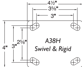
* Attaching Bolt Size For Plate 3/8" (Formerly 125)
