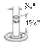
437SX1 5/16 Stem
