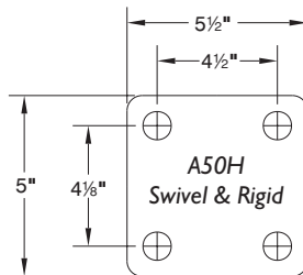
* Attaching Bolt Size For Plate 1/2" (Formerly 125E)
