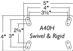
* Attaching Bolt Size For Plate 3/8" (Formerly 125B)
