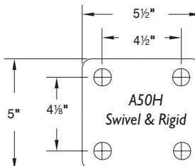
* Attaching Bolt Size For Plate 1/2" (Formerly 125E)
