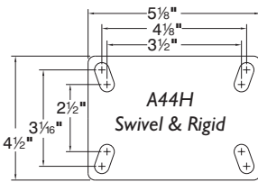
* Attaching Bolt Size For Plate 3/8" (Formerly 125F)
