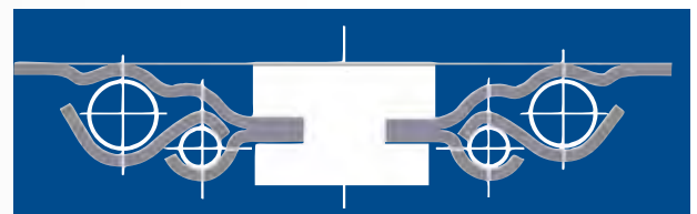
200 Series Swivel Cross Section
