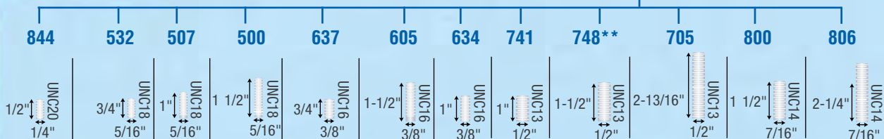
Tread Lock Brake 4" and 5" models. Add [-B] at end of model.
