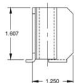
Inside Angle Welded (1G000220694) Raw (unplated) Finish
